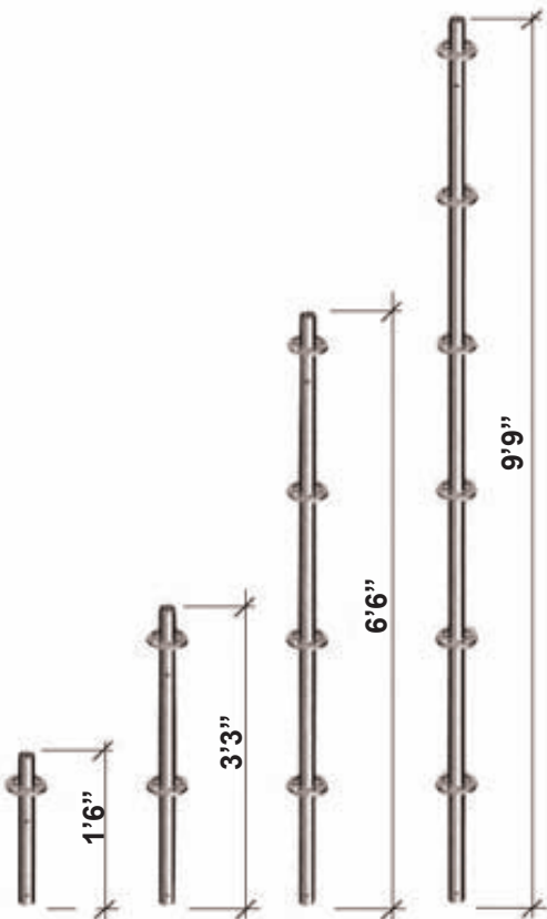
SYSTEM POSTS
