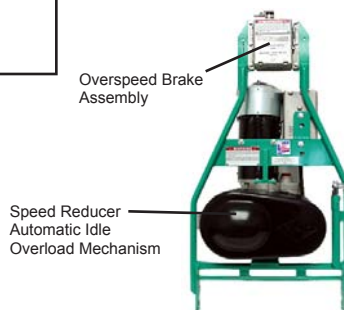
Powered Hoist
